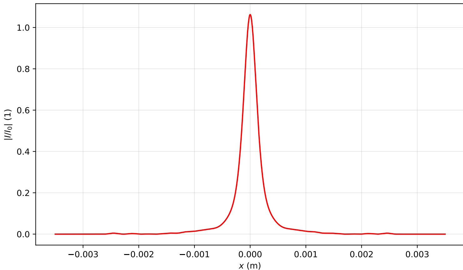
Intensity profile I(x, y = 0, z = 3.025)/I_0 , P_{in}=4.0P_{cr} , artificial time
